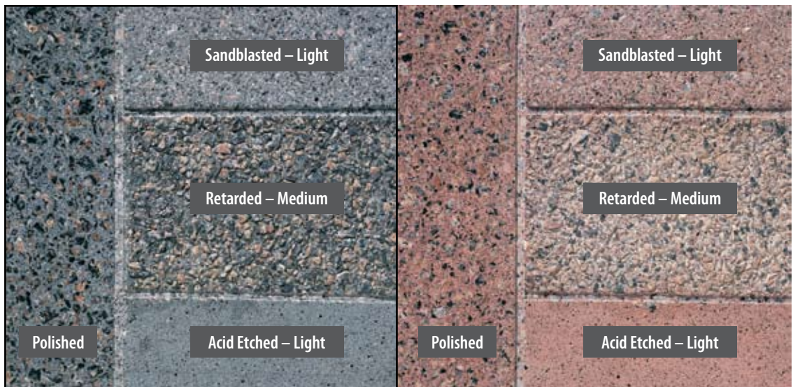
Figure 1 Appearance variations are achieved with different finishes on the same concrete mixture. (Courtesy Architectural Precast Concrete)
